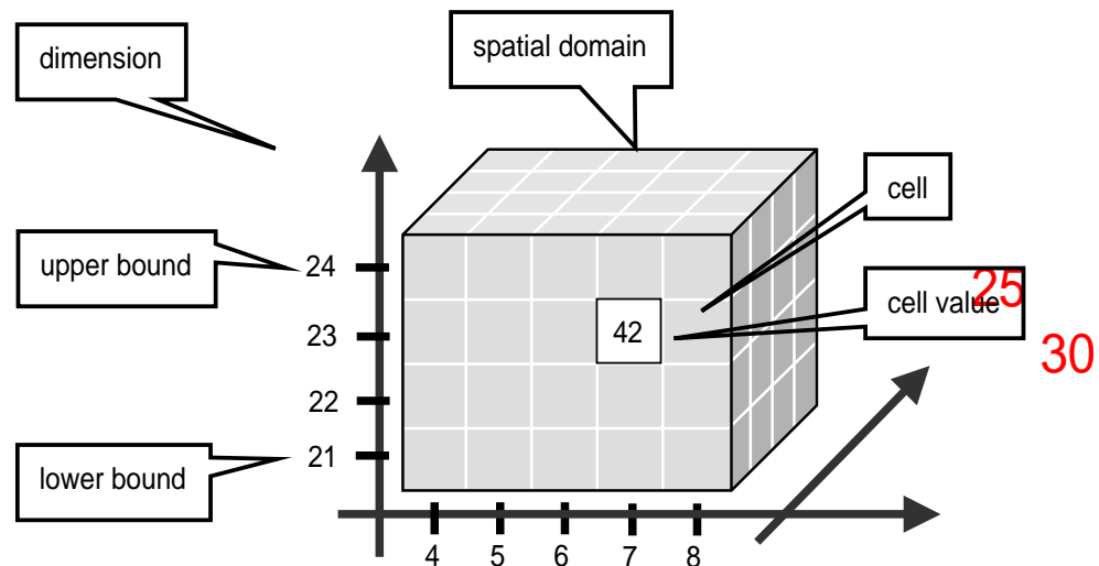
Figure 3 Constituents of an array
