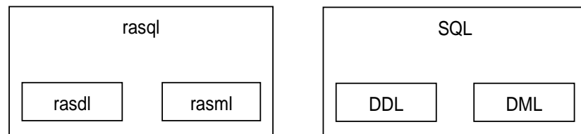
Figure 2 Correspondence between rasql and SQL
