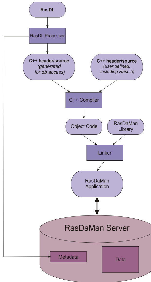
Figure 7 Application development workflow
